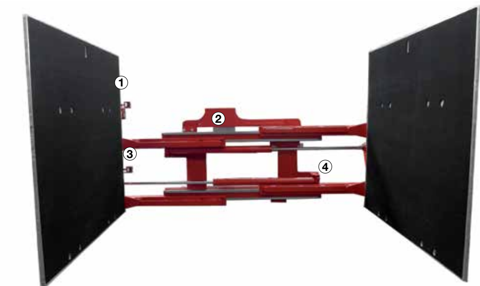
1 Laser detector Laser sensor for upper row to detect presence of boxes in the upper part of the pads.
